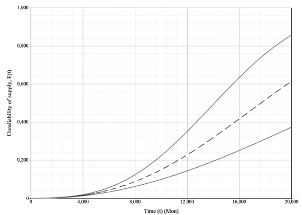
Fig. 3. Unreliability of supply vs. time plot.
